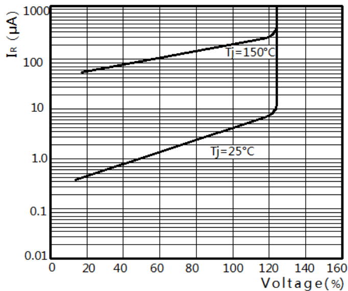
FIGURE 2. REVERSE CURRENT vs REVERSE VOLTAGE
