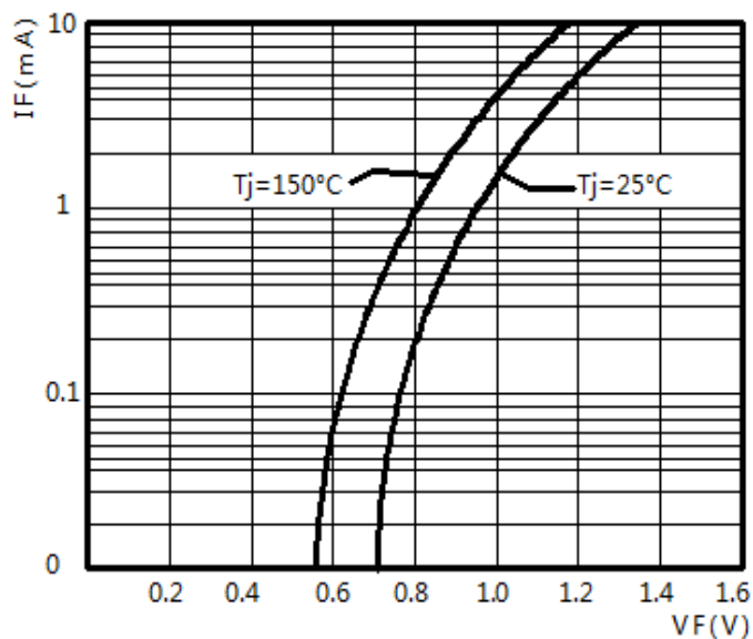
FIGURE 1. FORWARD CURRENT vs FORWARD VOLTAGE
